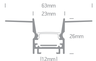
7903TR/B | 2m Trimless profile + PC opal diffuser | Aluminium | Suitable for 7820 LED Strip 12mm
