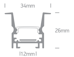
7903TR/W | 2m Trimless profile + PC opal diffuser | Aluminium | Suitable for 7820 LED Strip 12mm
