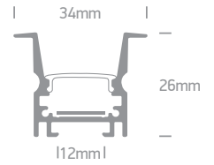
7903R/W | 2m Recessed profile + PC opal diffuser | Aluminium | Suitable for 7820 LED Strip 12mm
