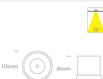
Suitable for 89030C driver.
