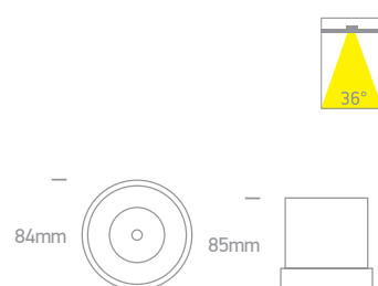
Suitable for 89015A driver.
